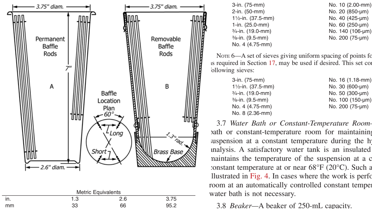
FIG. 2 Dispersion Cups of Apparatus
